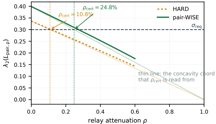
(b) why the budget is certified: \lambda_2 is concave in \rho
