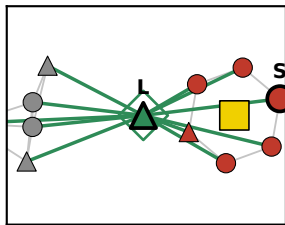
(c) WISE: long relays ( \lambda_2 = 0.78 )
