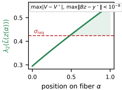
(a) certified fiber (dim E = 59 )
