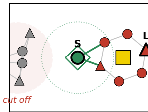
(b) long lifts ( \lambda_2 < 10^{-8} )
