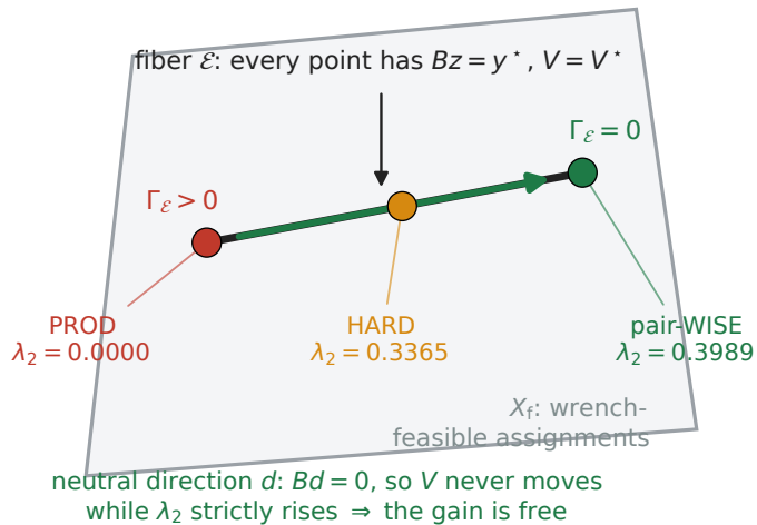
(a) the productive optimum fixes the aggregate, not the composition
