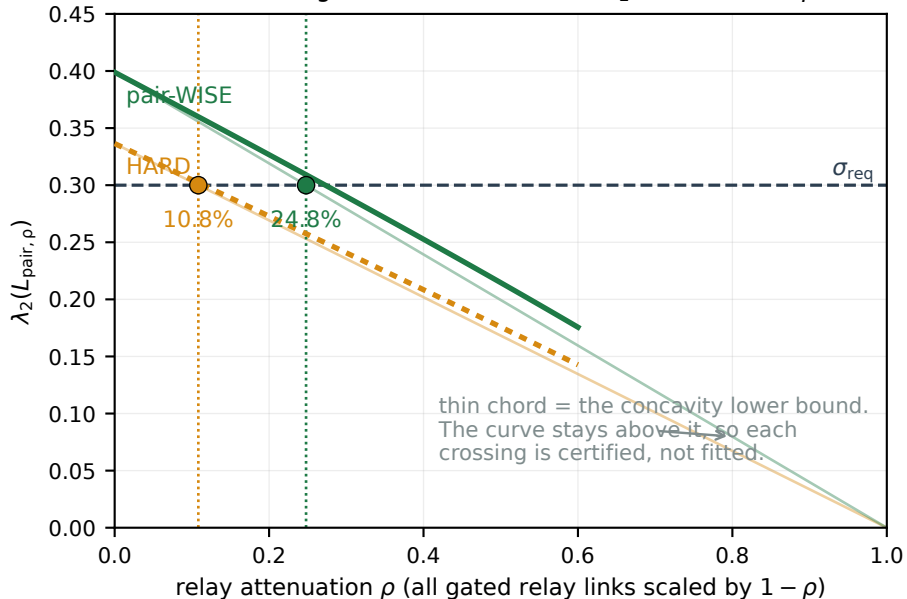
(b) the budget is certified because \lambda_2 is concave in \rho
