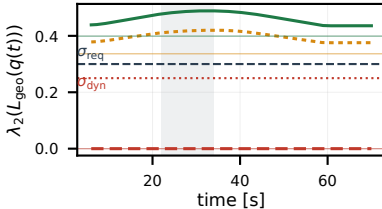
(b) realized vs. certified \lambda_2(\bar{L})
