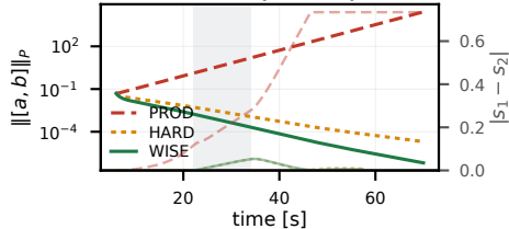
(c) information layer and sync. error
