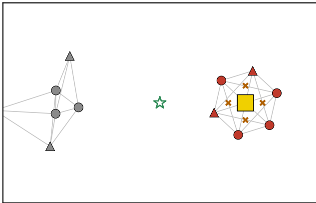
(a) productive-optimal, unsafe: \lambda_2(L_{\text{geo}}) = 0.00
