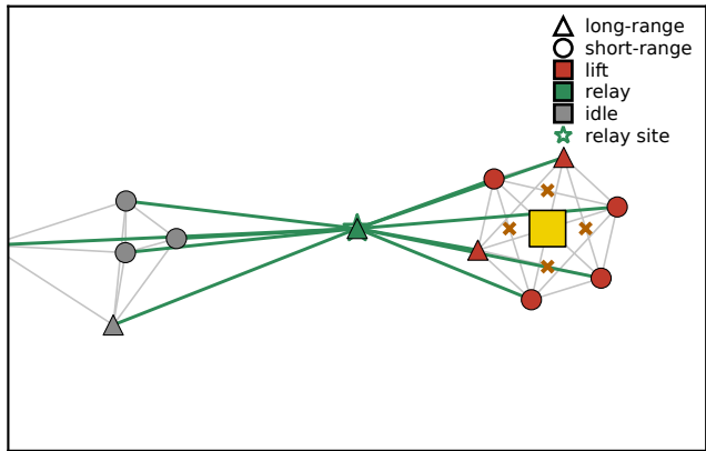
(b) WISE: \lambda_2(L_{\text{geo}}) = 0.85
