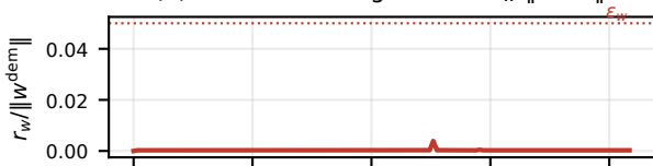
(b) wrench-tracking residual r_w / \|w^{\text{dem}}\|
