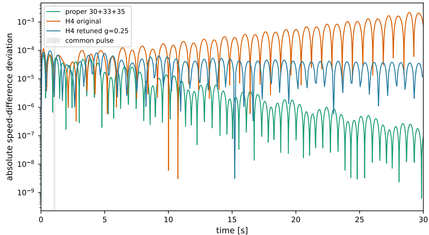
Equal-horizon TDS comparison: common +2% bus-20 pulse
