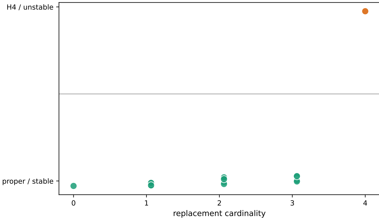
P2 — 15 safe proper portfolios, one unsafe full portfolio
