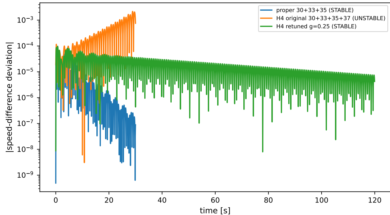
P8 — common +2% bus-20 load-pulse TDS
