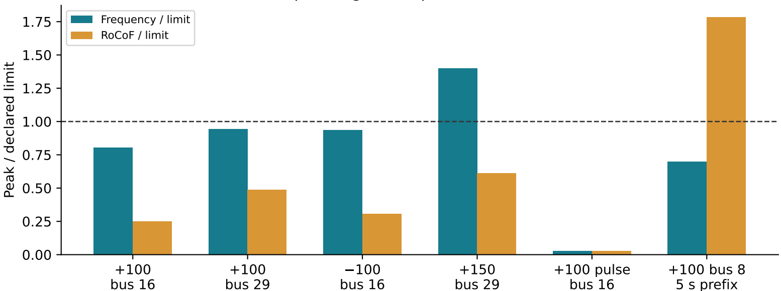
C Tested operating envelope; 150 MW is a stress test
