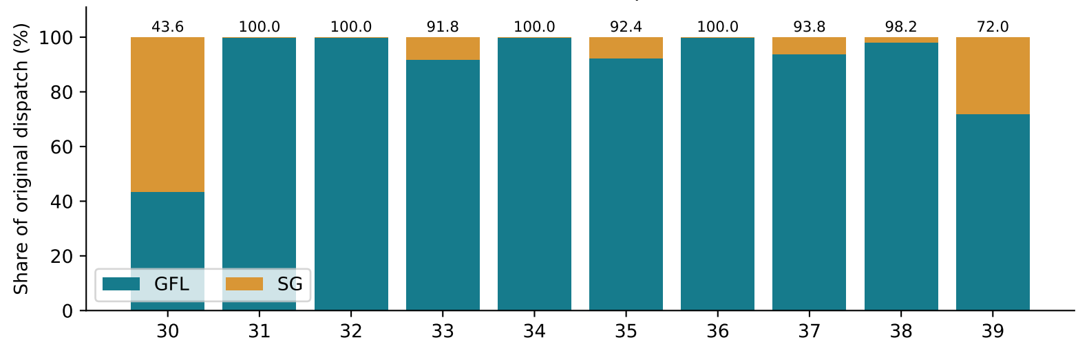
B Independent nonlinear PowerDynamics simulations
