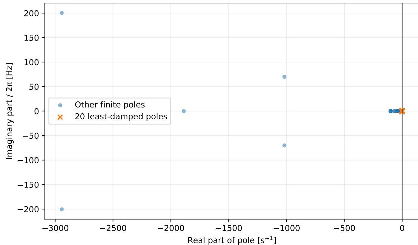
Full finite eigenvalue map
