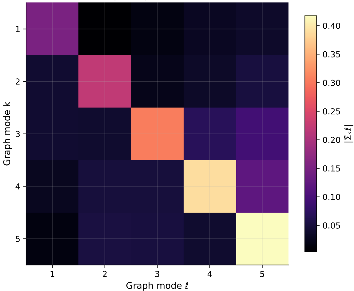
S2 |\hat{\Sigma}(j\omega)| at f = 2.1 Hz
