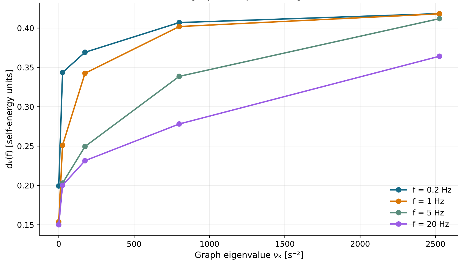
S2 graph dissipative diagonal
