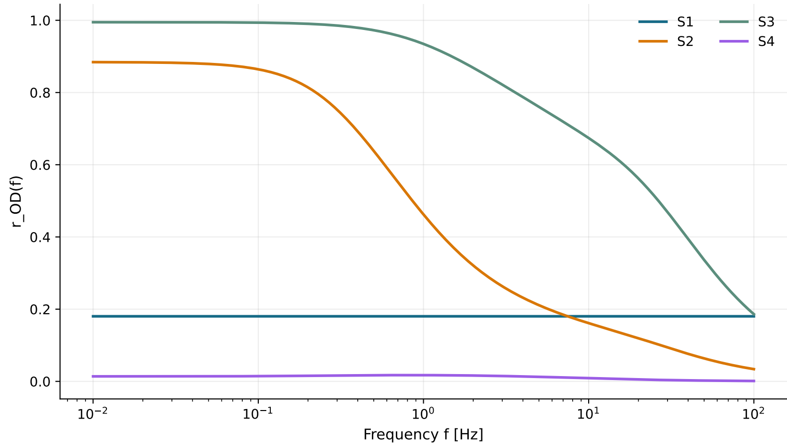
Off-diagonal graph self-energy ratio
