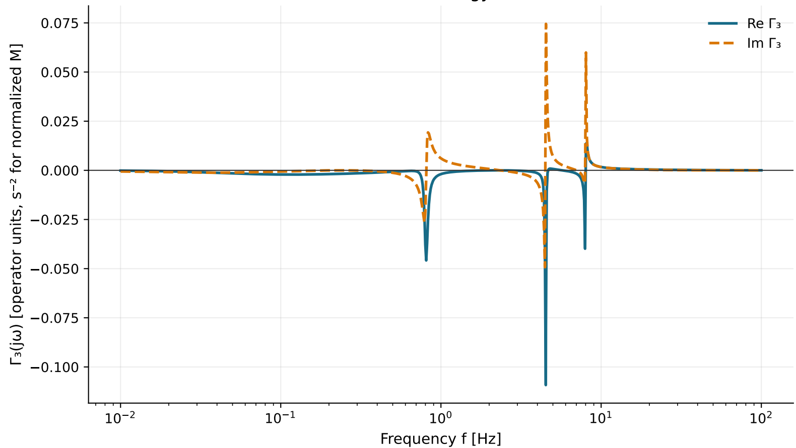
S2 collective self-energy, mode k = 3
