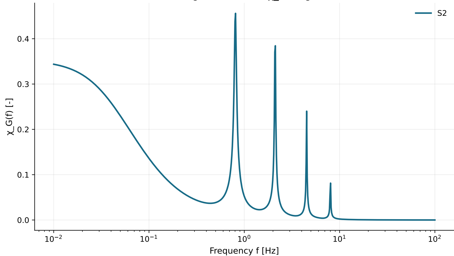
S2 finite-grid candidate \chi_G diagnostic
