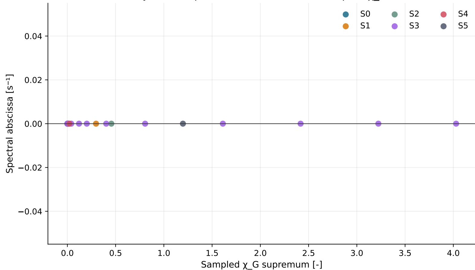
Synthetic spectral abscissa versus sampled \chi_G
