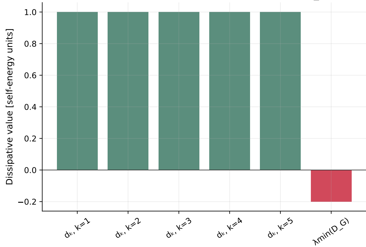
S5 positive diagonal entries with indefinite D_G
