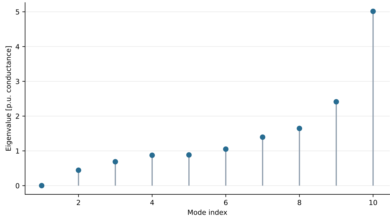
Spectrum of the passive generator-port graph
