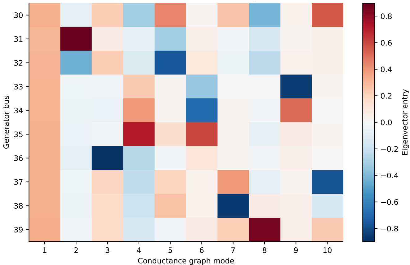
Euclidean eigenvectors of L_c = \Re(Y_{port})
