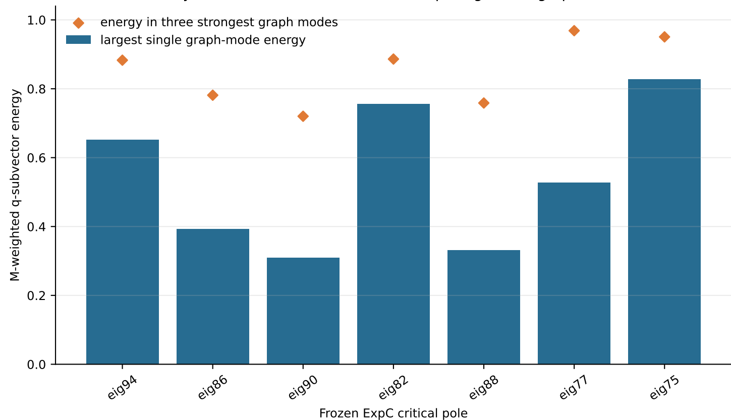
Physical critical-mode content in the preregistered graph basis
