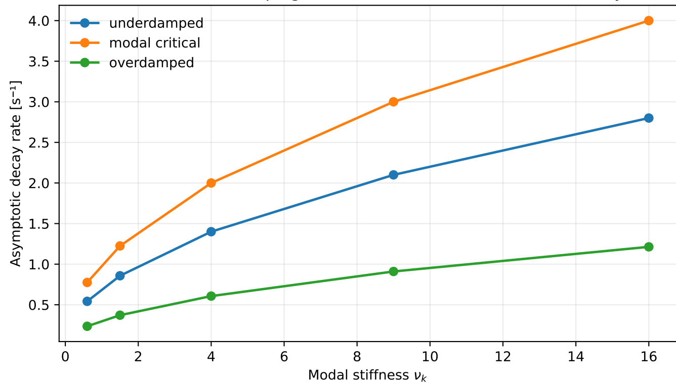
Critical modal damping maximizes each isolated mode's decay
