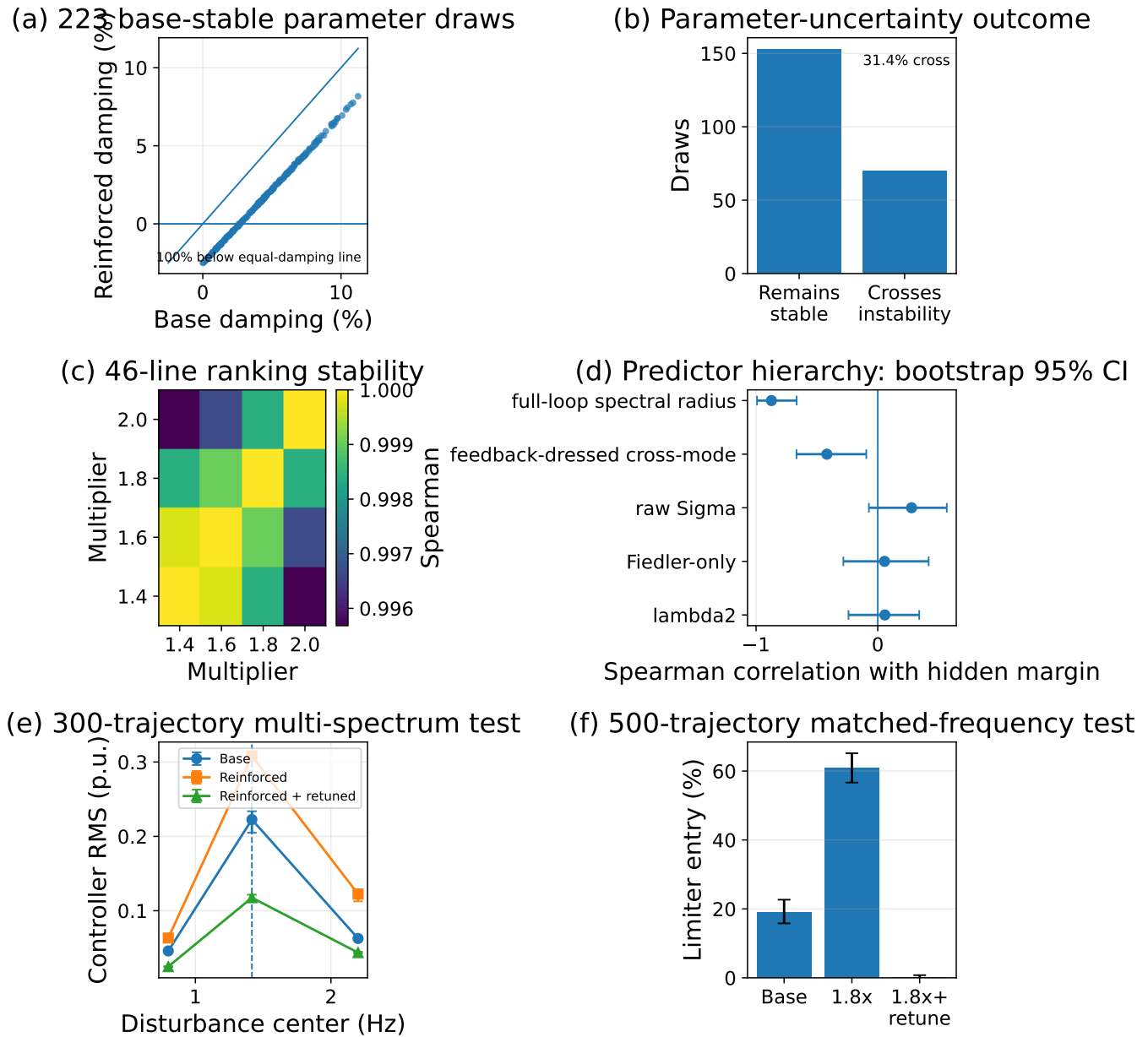
Fig. 6. Statistical and nonlinear falsification tests. (a) Reinforced versus base damping for the 223 parameter draws that are base-stable; all lie below the equal-damping line. (b) Of these draws, 31.4% cross instability after the same physical reinforcement. (c) Pairwise Spearman correlations of the 46-line hidden-margin ranking at four reinforcement magnitudes; all are at least 0.9957. (d) Bootstrap 95% intervals for the predictor hierarchy: only feedback-dressed cross-mode coupling and the full-loop spectral radius robustly exclude zero. (e) Controller-action RMS under 300-trajectory off-resonance and near-critical stochastic tests, with bootstrap confidence intervals. (f) Independent 500-trajectory matched-frequency limiter-entry experiment with uncertainty bars. The panels combine parametric, ranking, statistical, spectral, and nonlinear stress tests.
