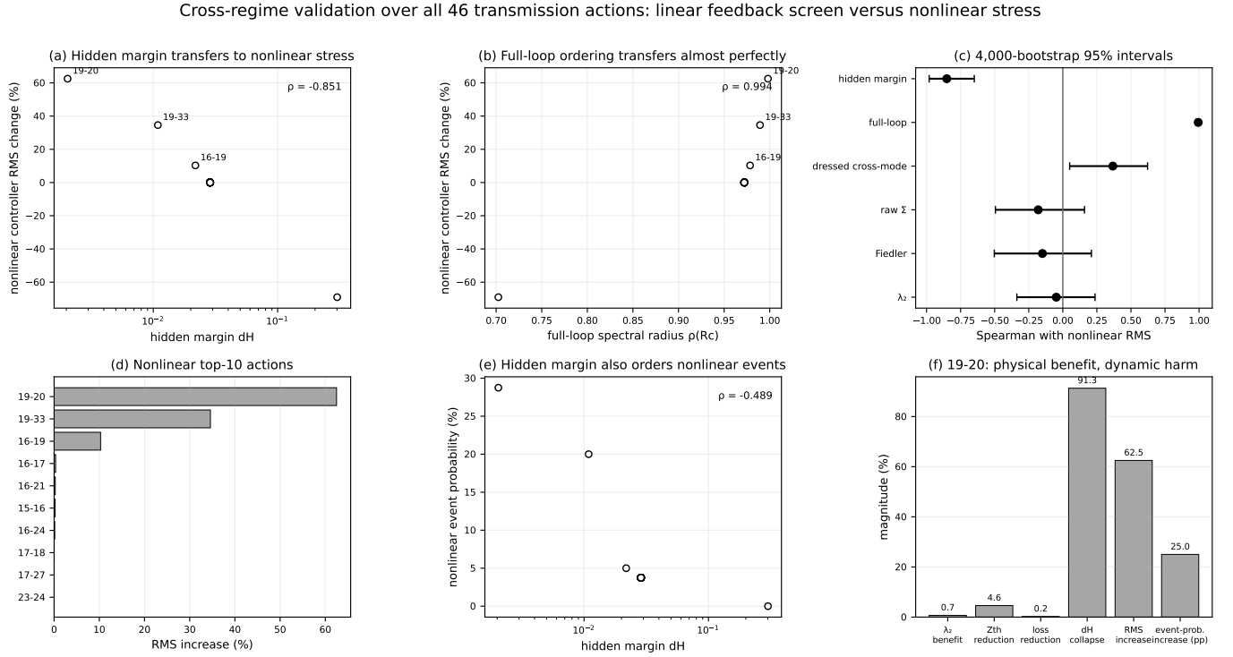
Fig. 7. Complete 46-action cross-regime nonlinear validation. (a) Hidden feedback margin versus nonlinear controller-action RMS change under an identical broadband OU disturbance for every reinforced branch. (b) Full-loop spectral radius versus the same nonlinear response; the ranking transfers with \rho = 0.994 . (c) Four-thousand-bootstrap 95% intervals for correlations with nonlinear RMS: physical \lambda_2 , Fiedler-only projection, and raw \Sigma are not statistically separated from zero, whereas feedback-dressed cross-mode coupling, full-loop spectrum, and hidden margin are. (d) The top ten nonlinear stress amplifiers; the three actions frozen as dangerous by the linear screen remain the top three. (e) Hidden margin also orders nonlinear event probability. (f) The 19–20 star action summarized on a common scale: modest physical benefits accompany a 91.3% hidden-margin collapse, 62.5% RMS increase, and 25 percentage-point increase in event probability in this common broadband test.
