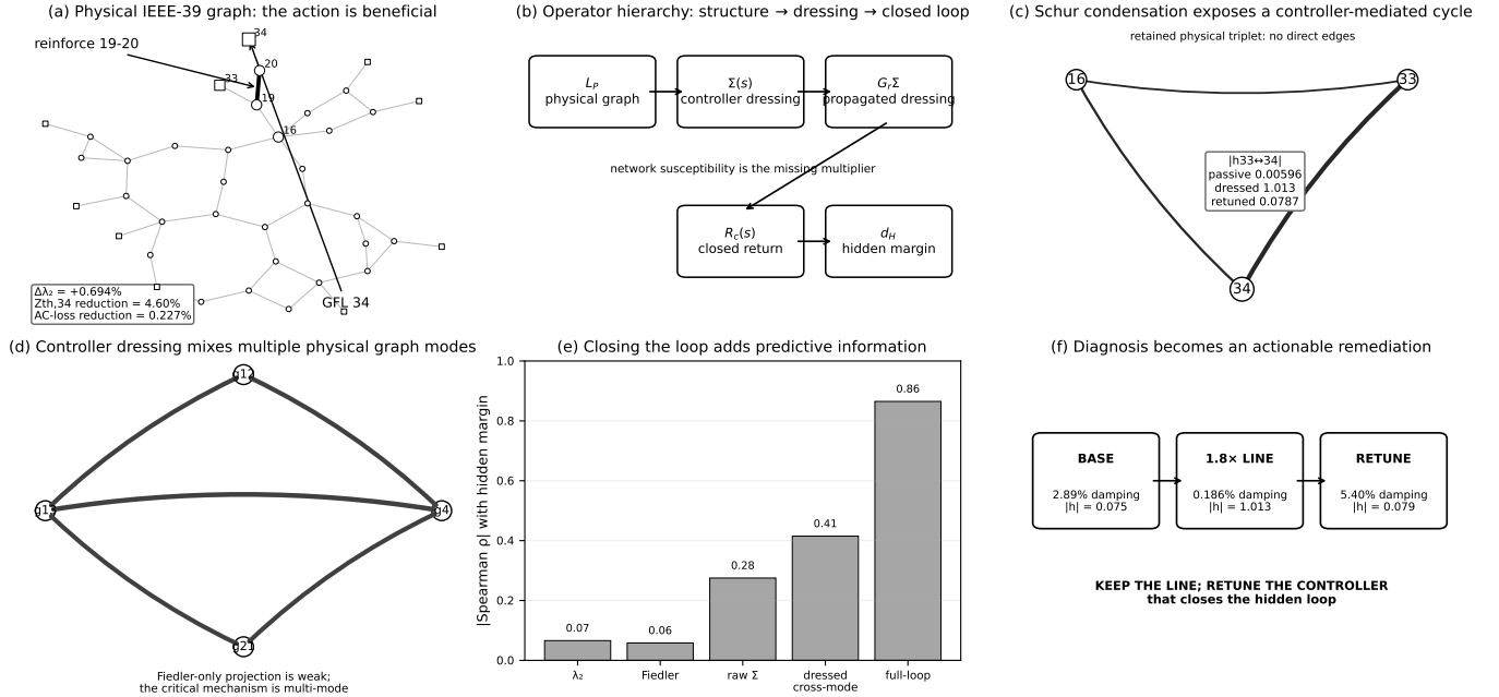
Fig. 1. Graphical summary of the proposed physical-to-dynamic hierarchy. (a) The IEEE 39-bus physical graph and the 19–20 star action are evaluated by AC quantities such as \lambda_2 , Z_{th} , and losses. (b) Controller self-energy is not used in isolation; network susceptibility propagates it through G_T\sigma before the controller-side return closes through R_c . (c) Schur condensation exposes effective edges and a controller-mediated cycle absent from the retained physical triplet. (d) The same dressing mixes several physical graph modes rather than only the Fiedler mode. (e) Empirical information increases as the loop is closed. (f) The resulting diagnosis is actionable: retain the physically useful reinforcement and retune the controller that closes the hidden loop.
