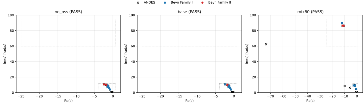
Figure 8: Phase-0D NEP contour validation: ANDES poles, NEP zeros, control poles, and contours.
