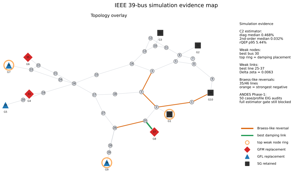
Figure 11: IEEE39 result-map artifact.
