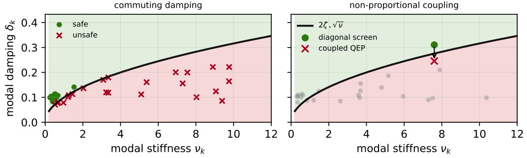
Figure 1: Damping-region geometry from the full manuscript.
