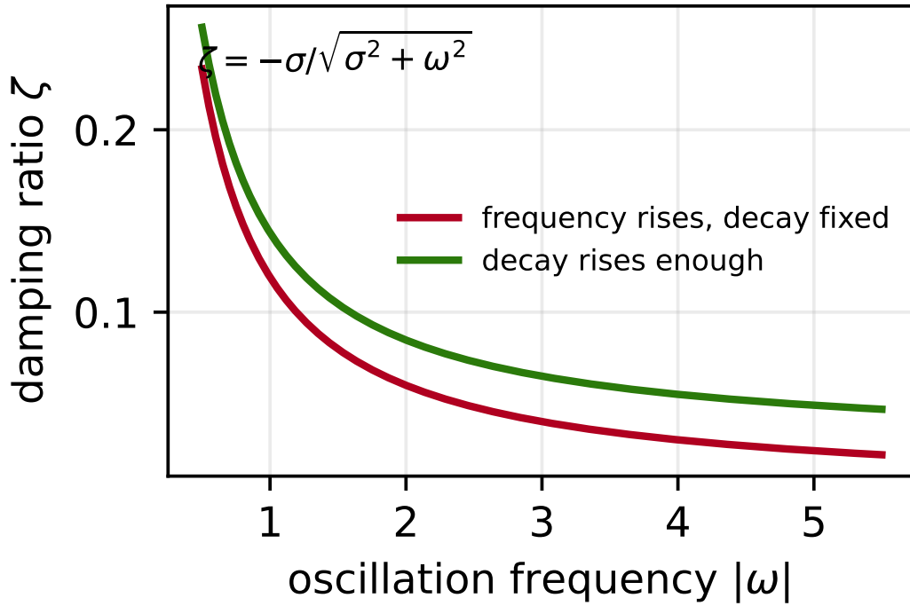
Figure 4: Frequency-only versus damping-aware line reinforcement tradeoff.
