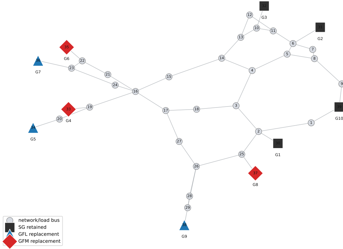
Figure 5: IEEE39 SG-to-IBR replacement map.
