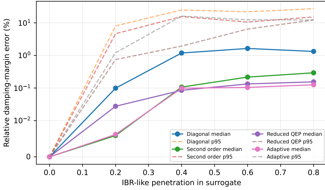
Figure 12: Estimator errors by IBR penetration in the rational-filter artifact set.
