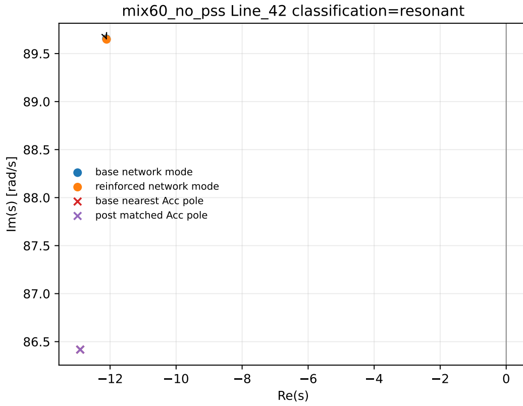
Figure 7: Control-resonant Braess example in the complex plane.
