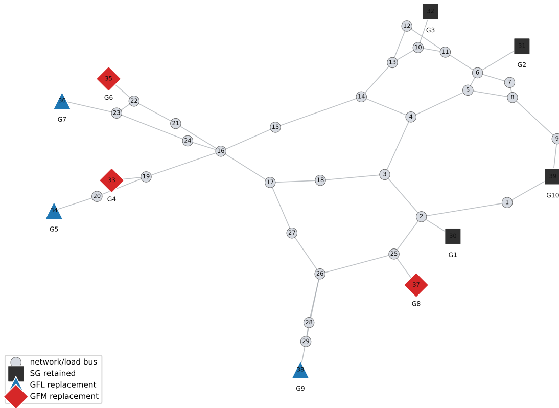
Figure 10: Mix60 IBR map generated during the ANDES bridge phase.
