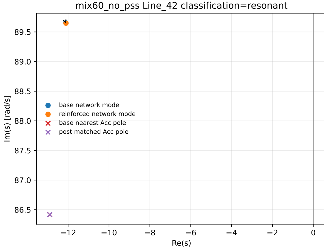
Figure 9: Phase Braess-NEP resonant line-reinforcement witness.
