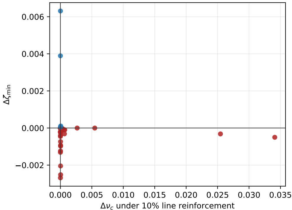
IEEE39-derived surrogate line reinforcements
