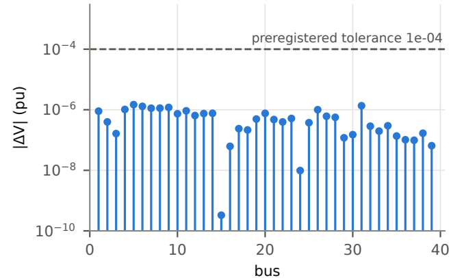
(a) voltage-magnitude residual
