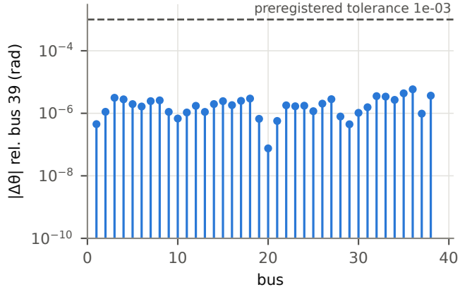
(b) voltage-angle residual
