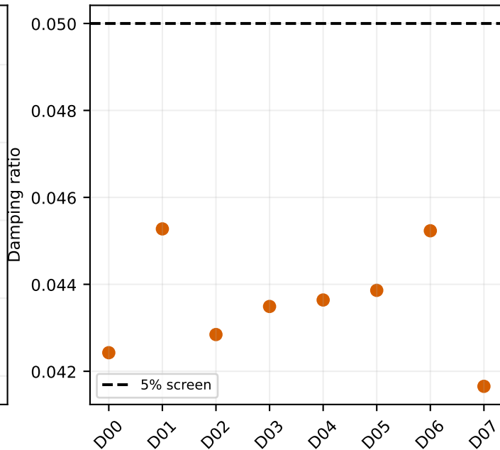
Margin-setting mode damping
