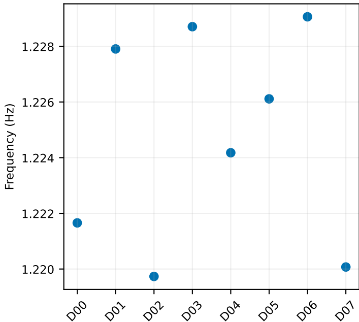
Margin-setting mode frequency
