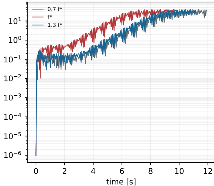
44 ms, no retune: PLL error [deg]
