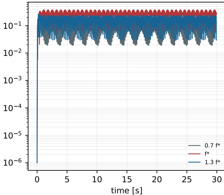
40 ms baseline: PLL error [deg]
