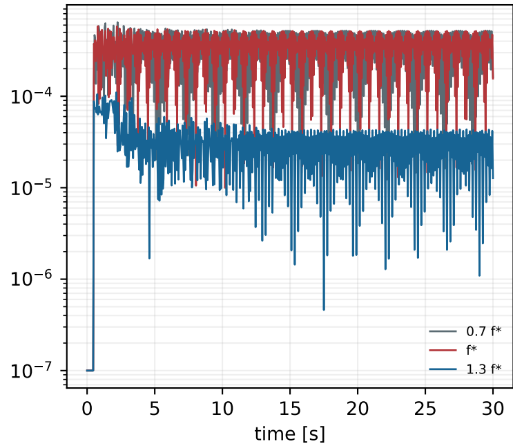
all-SG: bus-frequency dev [Hz]
