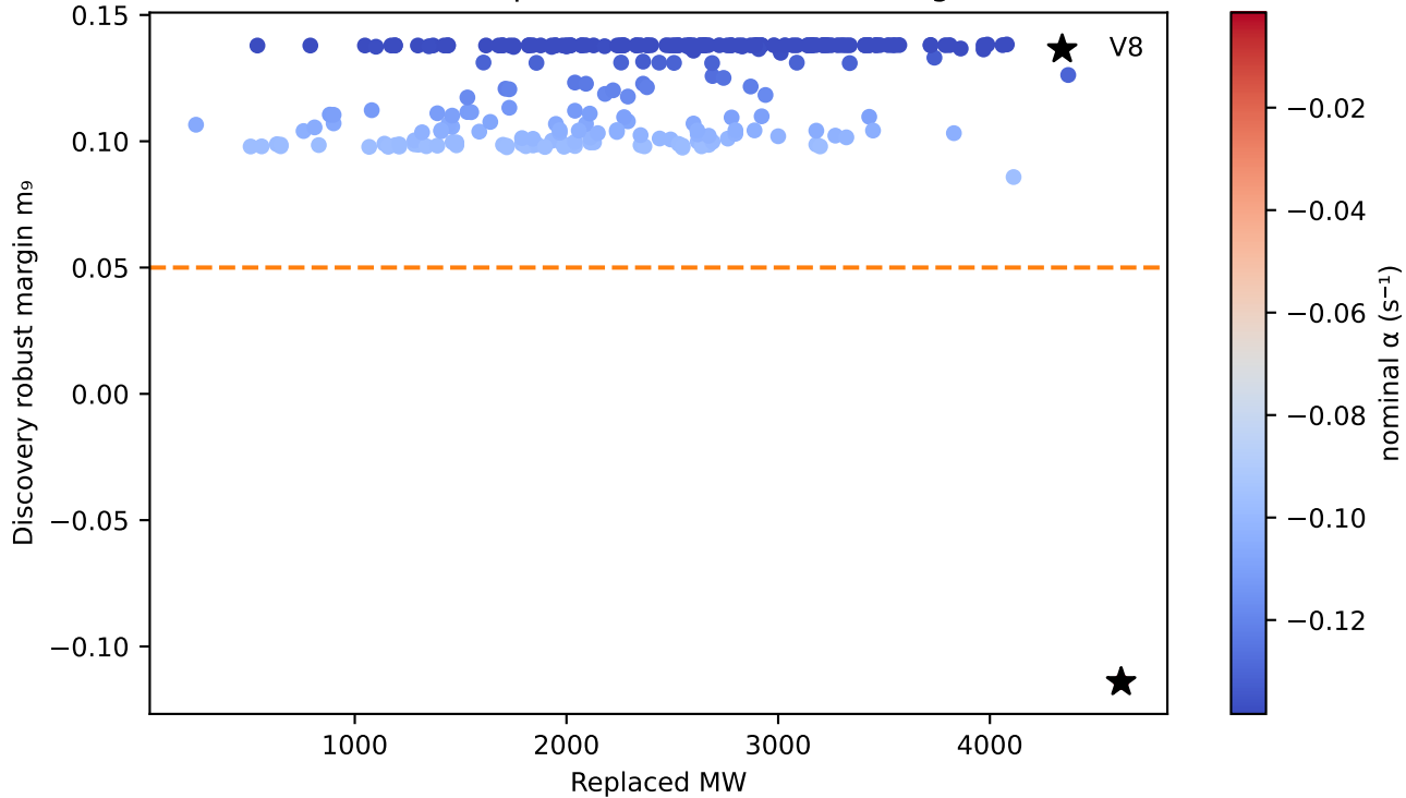
F10 — IBR penetration vs robust margin
