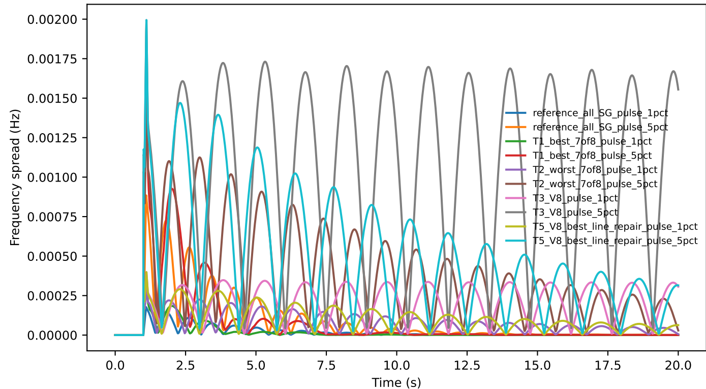
F12 — TDS common-disturbance frequency spread
