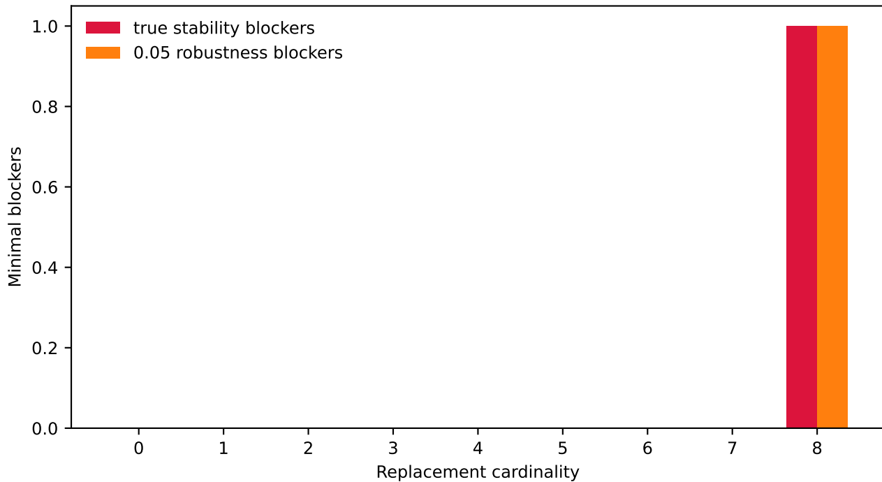
F2 — 255 + 1 structure (exact finite benchmark)
