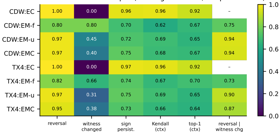
P4 core lattice under envelopes (coverage fractions, not probabilities)
