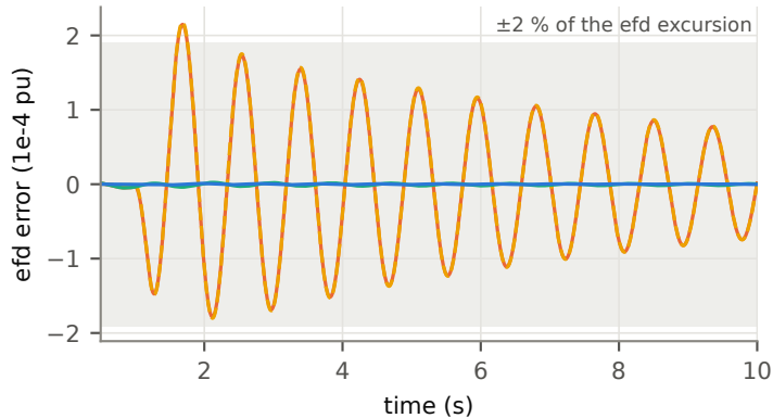
(a) AVR-state error after the Pm pulse
