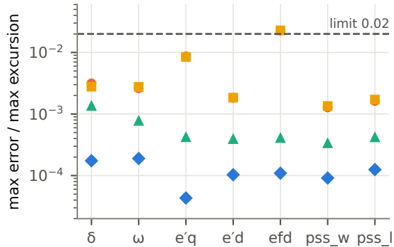
(b) all seven states
