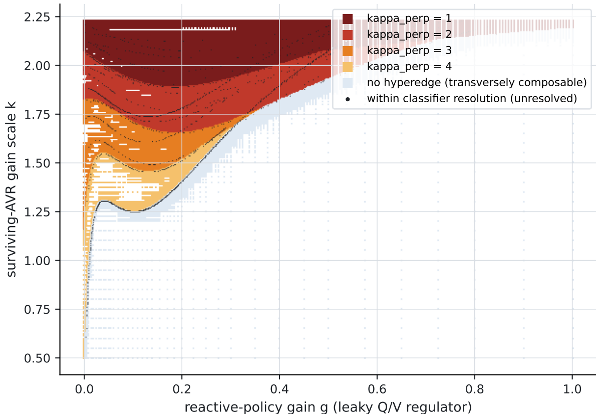
Transverse incompatibility order kappa_perp over the policy plane IEEE-39, F7A slice (t = 1.5, h = 1), core 30/33/35/37, matched dispatch, no governor
