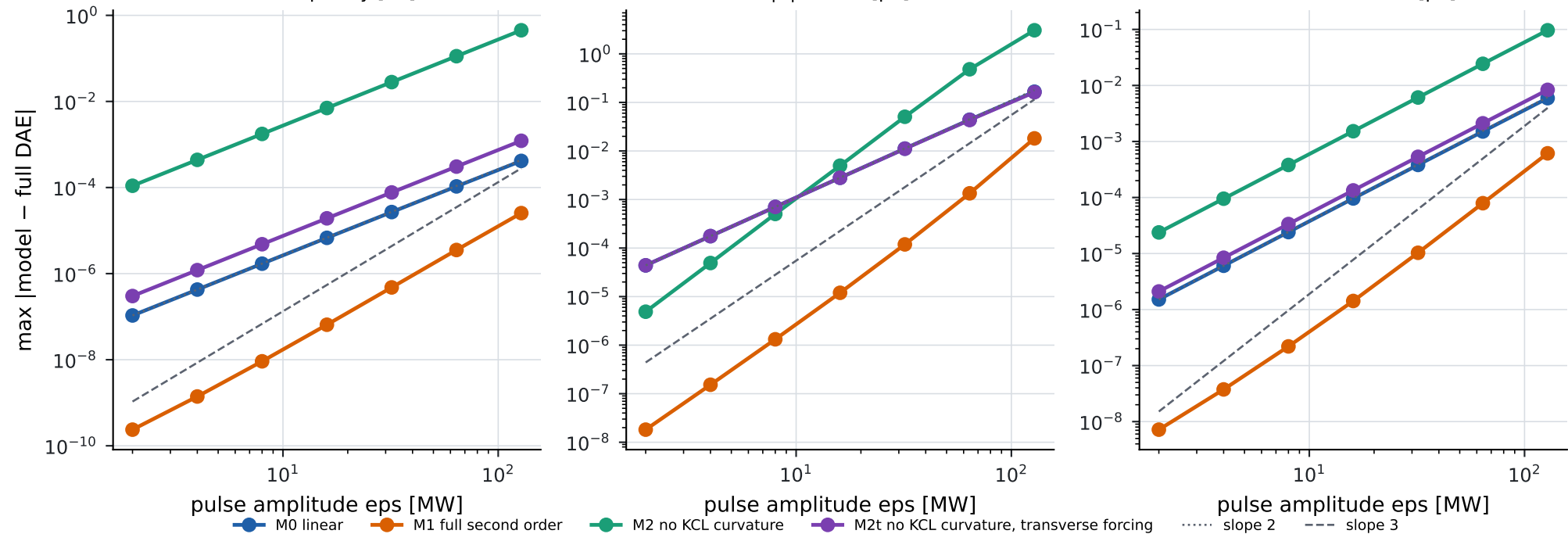
Second-order reduced response: linear (M0), full (M1), no KCL curvature (M2; M2t with transverse forcing) — critical triple 30+33+35 P4
