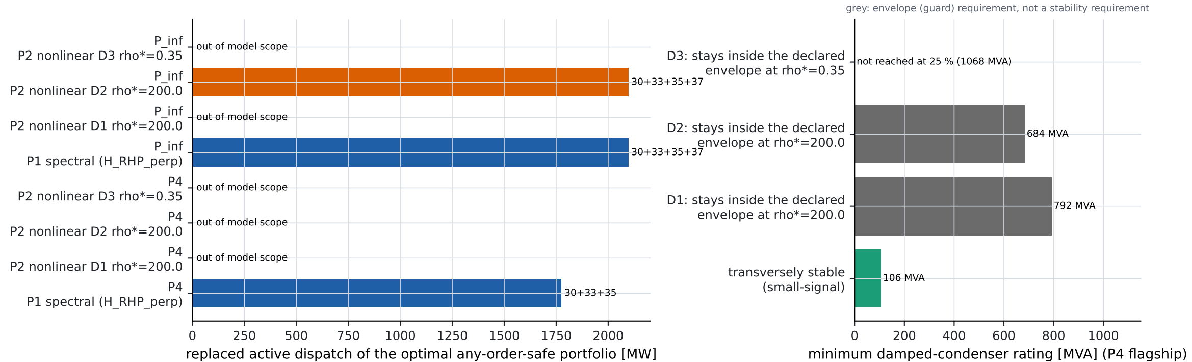
Planning: spectral-only vs nonlinear-safe vs support-assisted (MW and MVA on separate axes)
