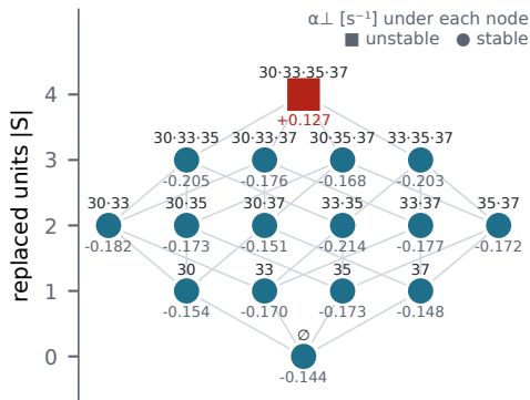
A P4 lattice: 15 proper subsets stable, H4 not
