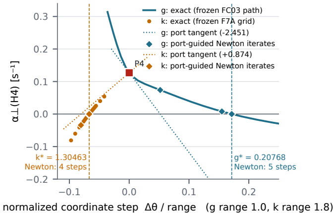
D Boundary motion: port derivative + Newton
