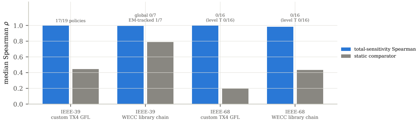
Cross-benchmark summary (text above bars: level-D reversal coverage)
