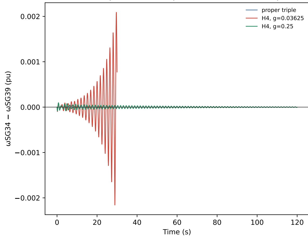
B Nonlinear phasor-DAE response to frozen 2% load pulse
