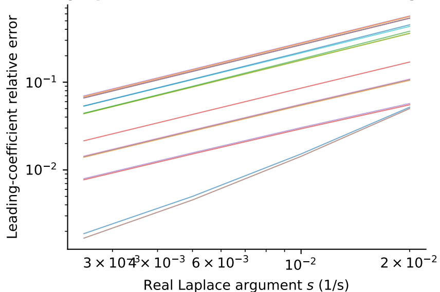
Asymptotic law, not a broadband surrogate
