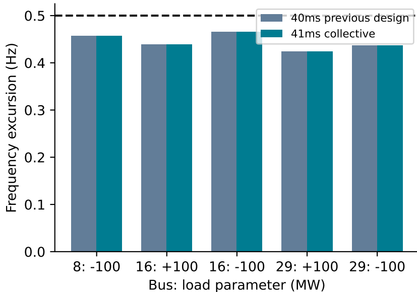
Frequency excursion (Hz)
