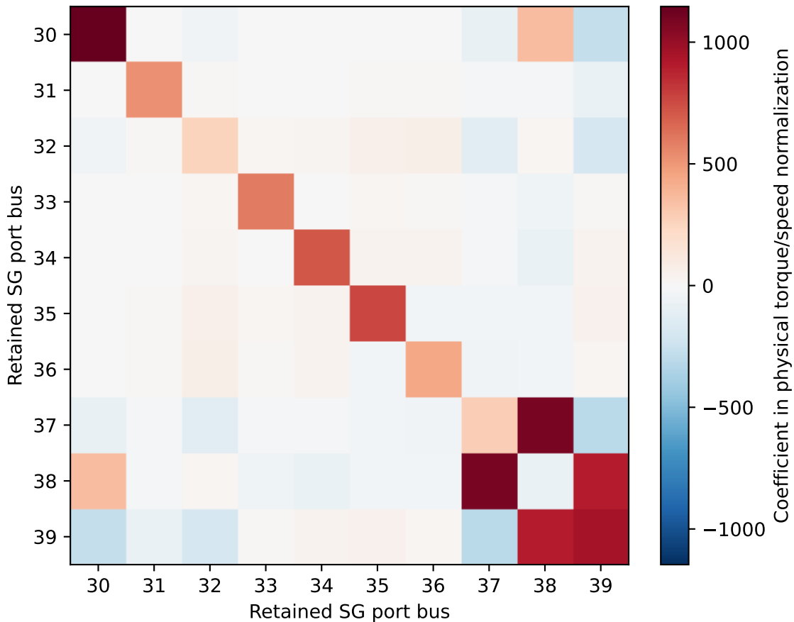
T, 45 ms: real part of physical Hermitian damping Frequency-specific operator; not a Laplacian
