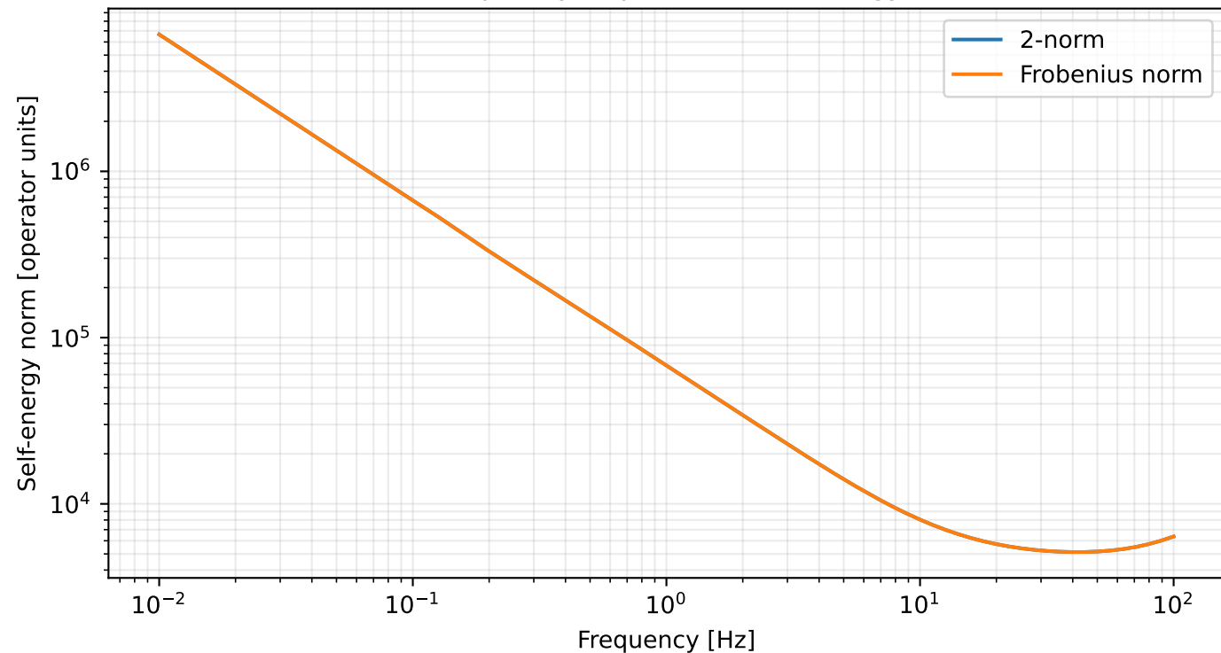
Frequency-dependent self-energy
