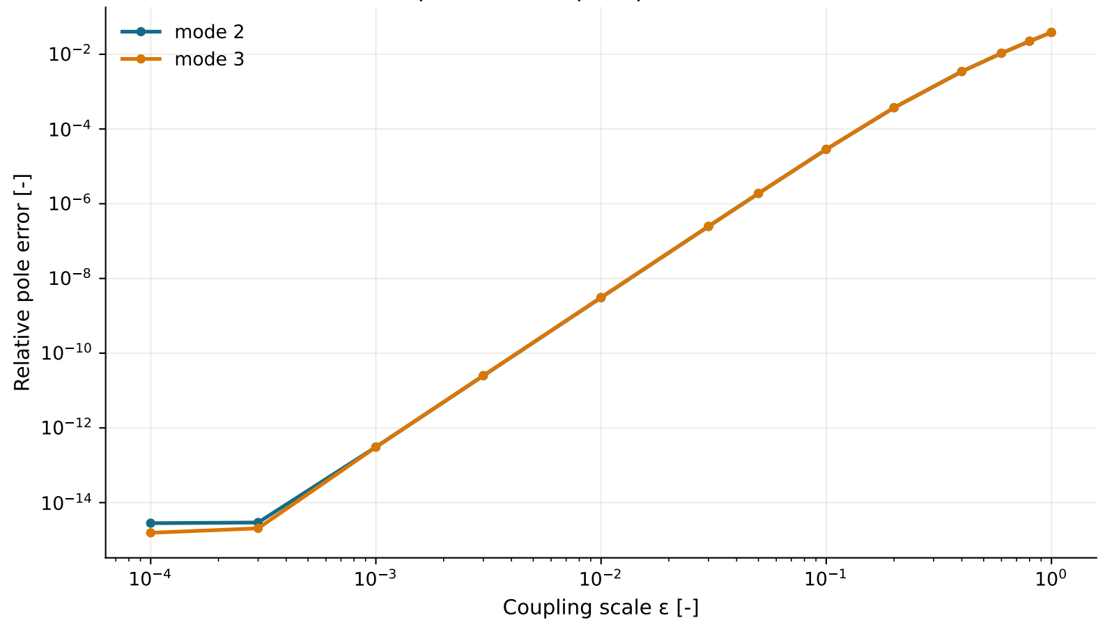
S3 perturbative pole prediction error
