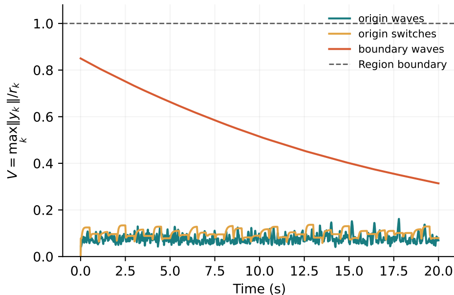
B Finite Julia checks of the pre-LP region
