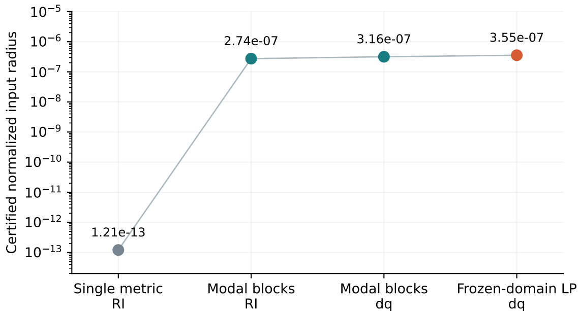
A Most improvement comes from modal comparison
