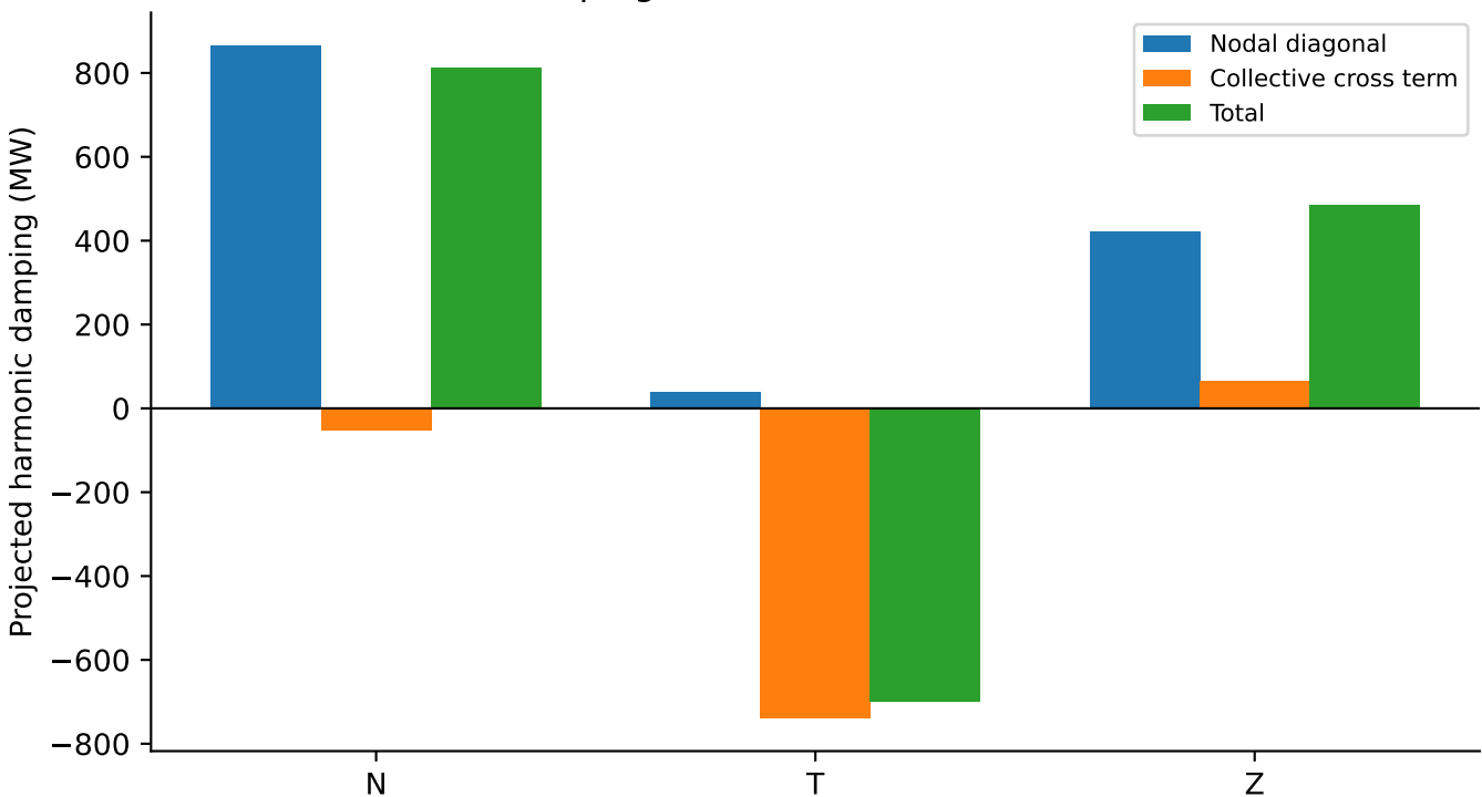
45 ms: damping on the tracked critical PLL motion
