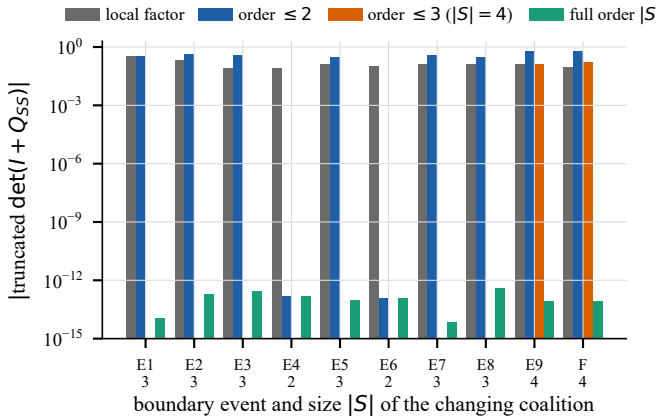
Fig. 5. Anatomy of the ten frozen IEEE-39 boundaries (E1–E9: F7B line t = 0.852 ; F: P4 line). Shown are the local factor and the truncations of the interaction expansion (9). Only the full-order term (order |S| ) reaches the characteristic zero. For pairs, order \leq 2 is the full order.
