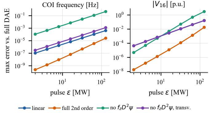
Fig. 11. Second-order reduced response of the triple 30+33+35 at P4 against the full DAE. The complete second-order model requires f_z D^2 \psi .
