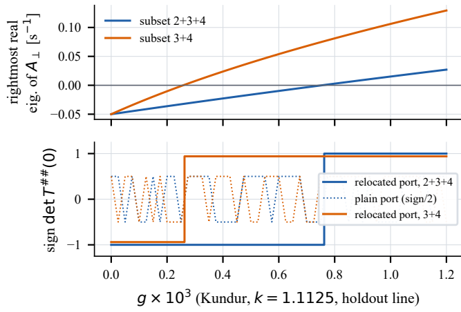
Fig. 8. Symmetry-deflated zero-frequency port on a Kundur holdout line. Top: the physical real transverse eigenvalue crosses zero. Bottom: the relocated port changes sign exactly at the crossings; the plain port (dotted) is structurally singular and its sign is numerical noise.
