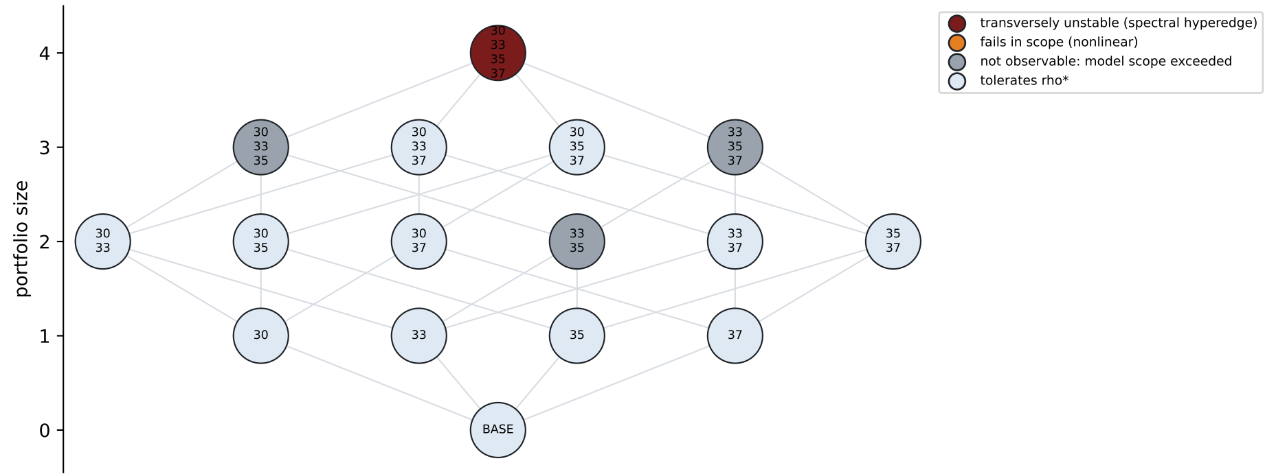
Spectral H_RHP_perp vs nonlinear status at \rho^* = 200 MW (D1, P4)
