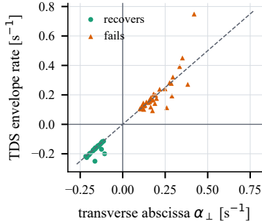
(b) nonlinear TDS, 5 MW pulse
