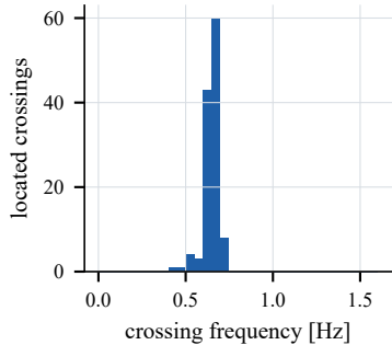
(c) crossings closing changes of \mathcal{H}
