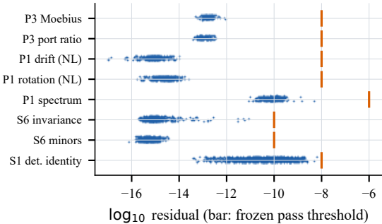
(a) exact identities
